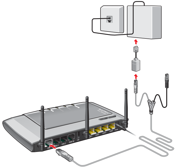
Connecting to the DSL splitter
