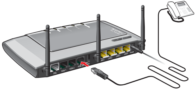
Connecting an ISDN telephone to the FRITZ!Box
